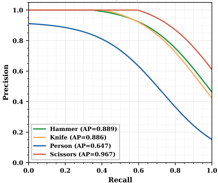
(a) Precision-Recall Curves Fine-tuned v5 (Final) — Test Set
